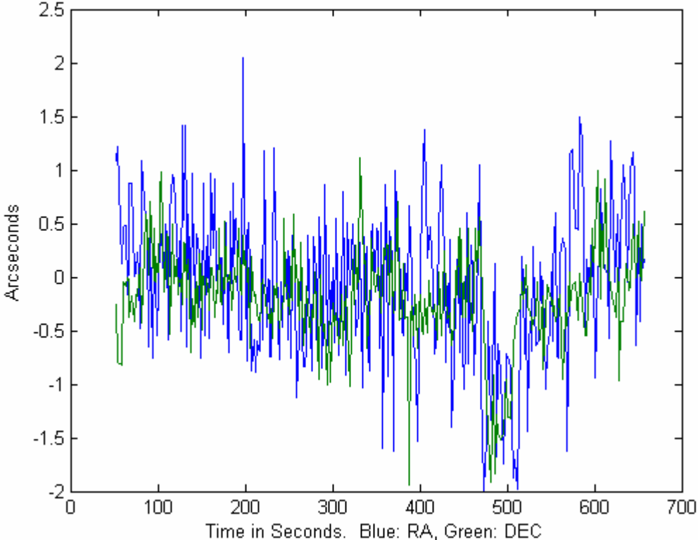
Periodic Error, C8-NGT, Guiding, Vega, East - 1" Heavy West, Alt PHd Settings (Std = 0.6604)
