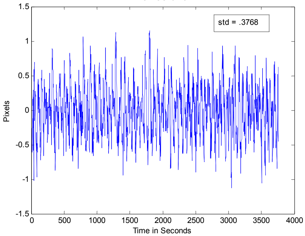
DEC NGC281 OIII
