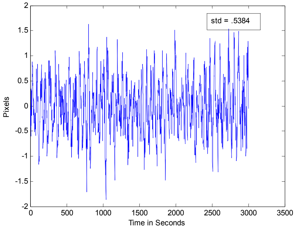
DEC NGC6960 SII
